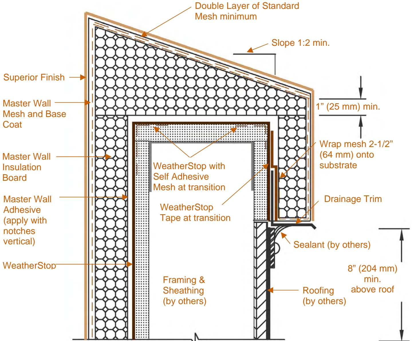
AFCD-24 Parapet Cap Detail – Max. 12" Wide
